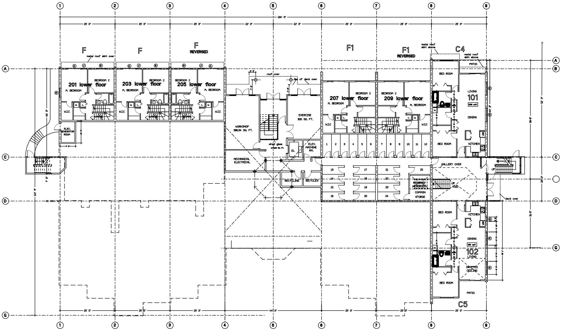
LOWER FLOOR LEVEL 9022 SQ. FT. lower floor area
